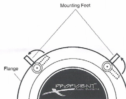
Diagram 5: Mounting Feet
