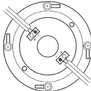
Diagram 4: Correct Polarity
